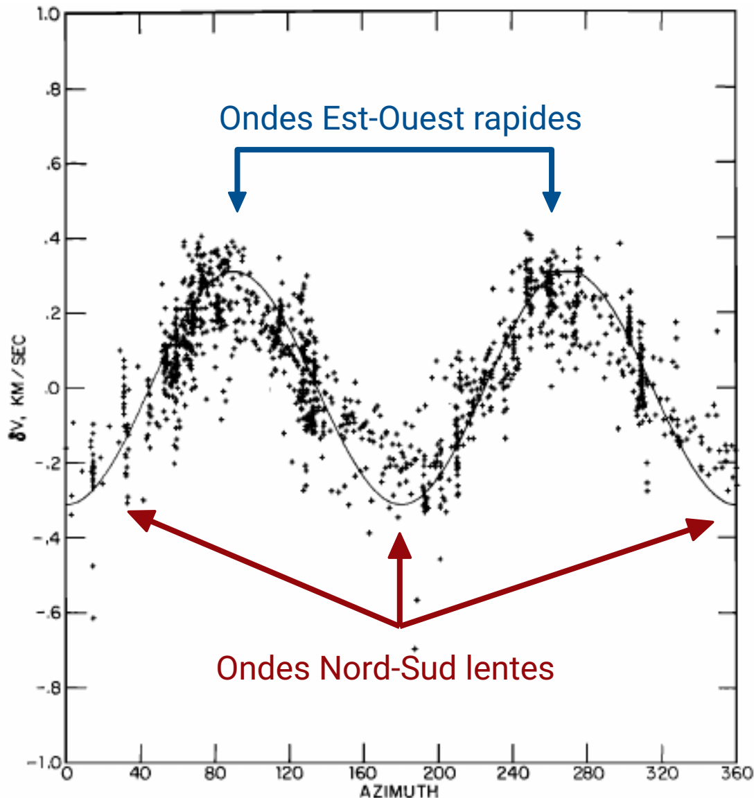
Fig. 12. Velocity anisotropy given as deviations from mean velocity of 8.159 km/sec plotted as a function of azimuth. Combined data are from Hilo and Show expeditions.
